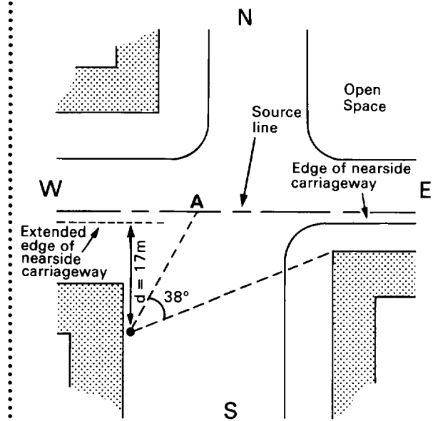
(iv) Segment E: d = 17\text{m} Angle of view = 38^\circ No reflecting facade opposite traffic stream
